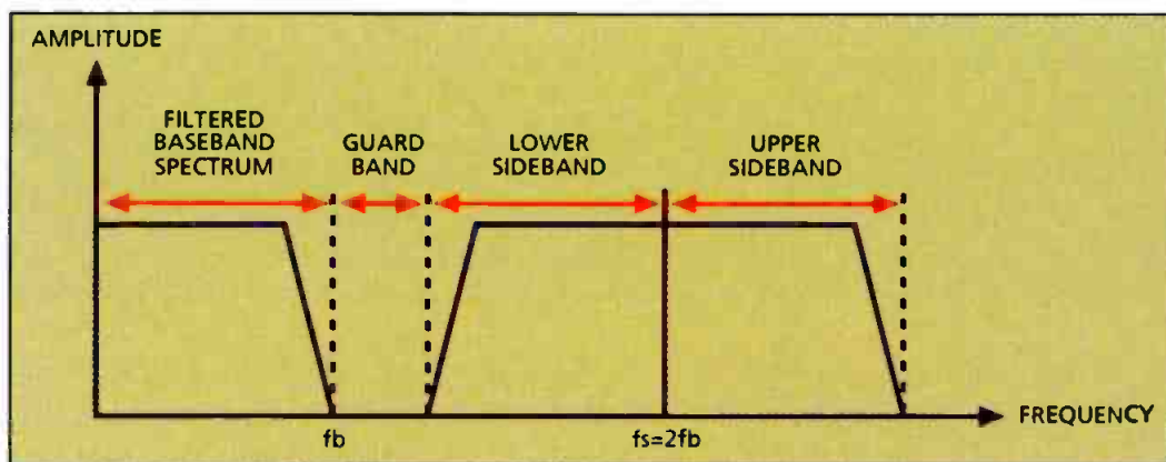
Figure 5: The spectrum of a sampled and filtered baseband signal.
